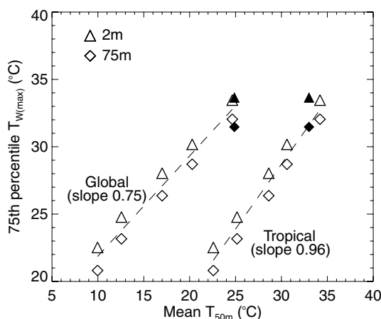
Fig. 2. The 75th percentile value of T_{W(\text{max})} (a measure of the peak occurrence value) at two or 75 meters above ground vs. global or tropical mean 75-m temperature in CAM3 simulations. Solid symbols are for a simulation representing possible Eocene conditions. Dashed lines show best linear fits, with slopes given (Eocene run not included in fit).
