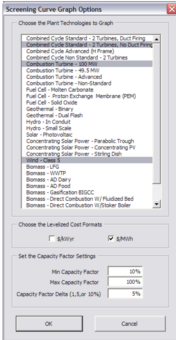
Figure A-7: Interface Window for Screening Curve
