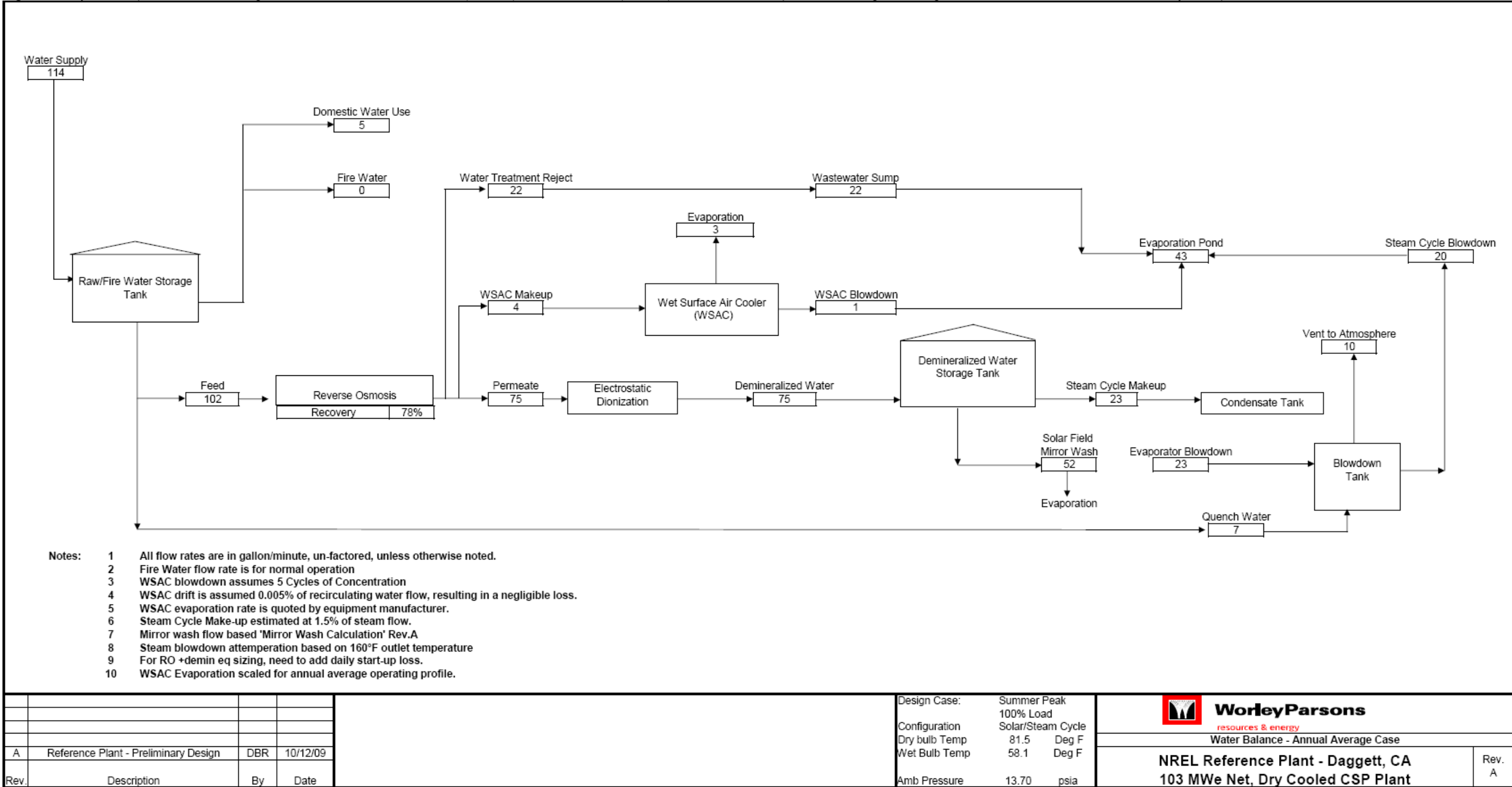
Figure 5. Dry cooled plant annual average case water balance at 81.5°F (27.5°C) DB and 58.1°F (14.5°C) WB ambient temperatures. Diagram is high-level and not inclusive of all water system processes.
