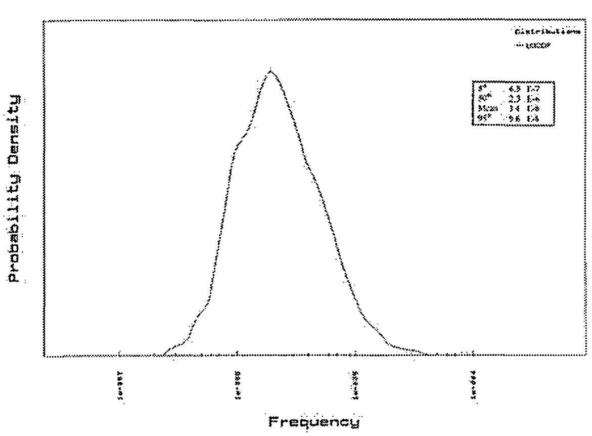
Figure 1-1 Uncertainty Curve for Browns Ferry Unit 3 Core Damage Frequency
