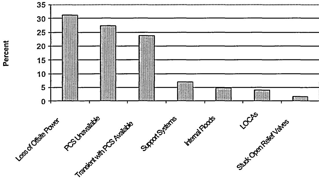
Figure 1-3 Browns Ferry Unit 3 Core Damage Frequency by Initiating Event Category
