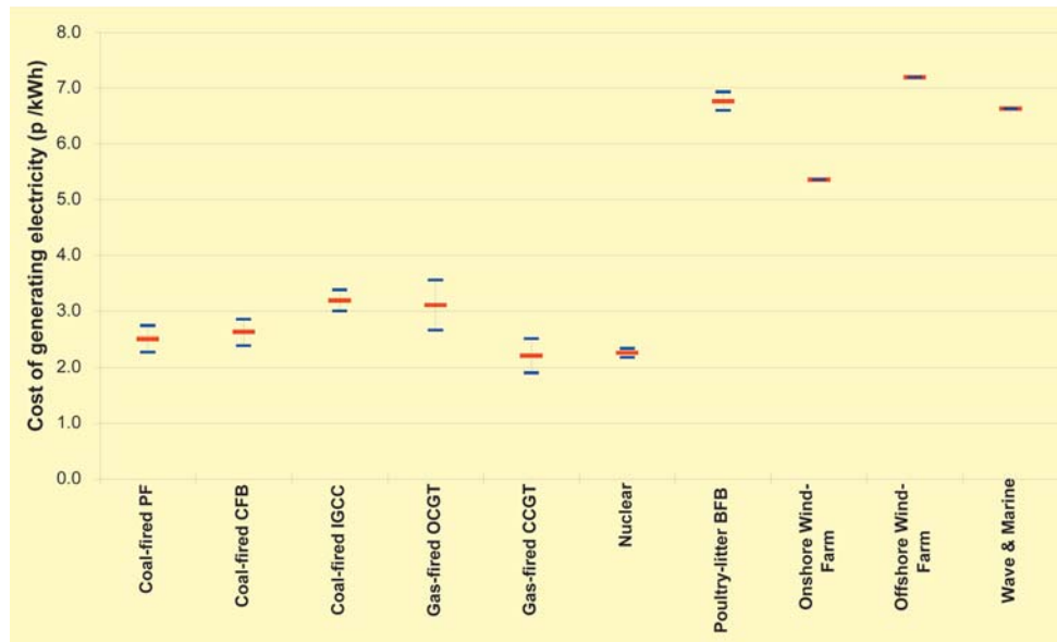
Figure 1.2 –Effect of ± 20% change in fuel price on the cost of generating electricity
