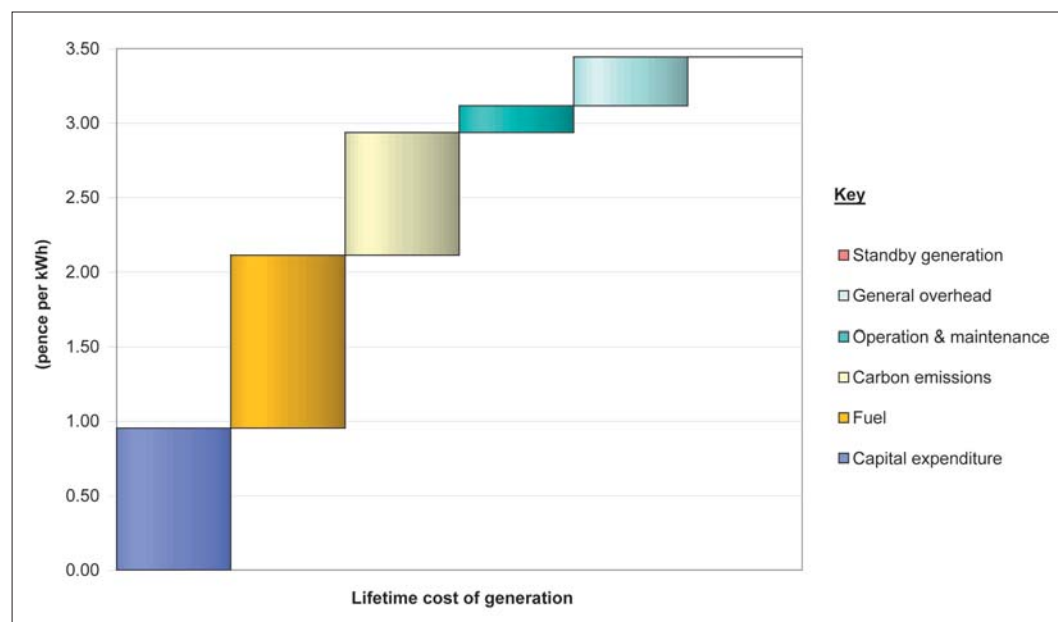
Figure A.2 – Current cost of generating electricity from coal-fired CFB plant
