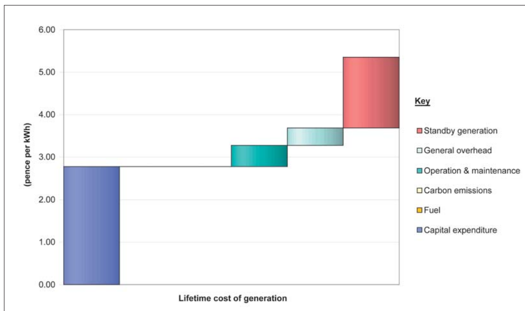
Figure A.10 – Current cost of generating electricity from an onshore wind farm
