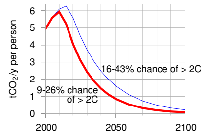
Figure 1.8. Global emissions for two scenarios considered by Baer and Mastrandrea, expressed in tons of \text{CO}_2 per year per person, using a world population of six billion. Both scenarios are believed to offer a modest chance of avoiding a 2^{\circ}\text{C} temperature rise above the pre-industrial level.
